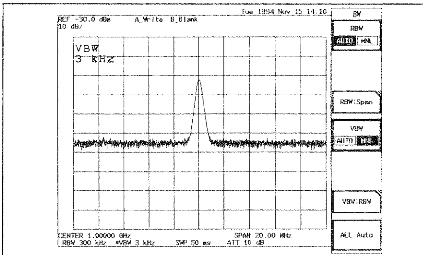
Figure 7-8 VBW = 3 kHz
