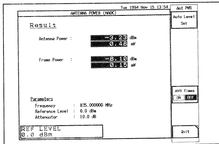
Figure 5-30 Antenna power measurement screen
