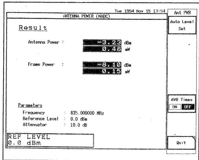
Figure 7-30 Antenna power measurement screen
