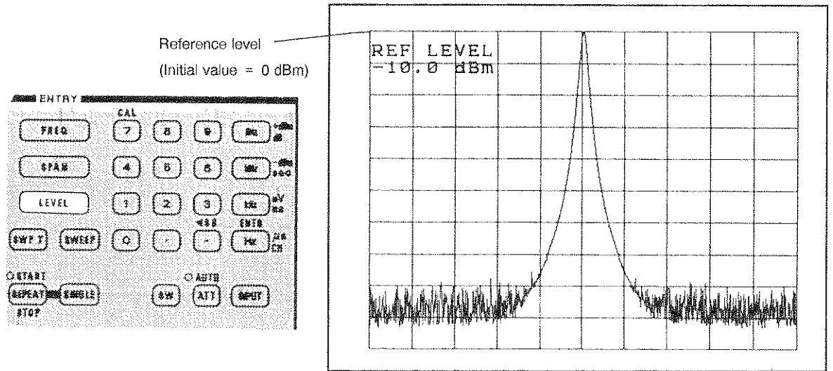
Figure 7-5 Reference Level
