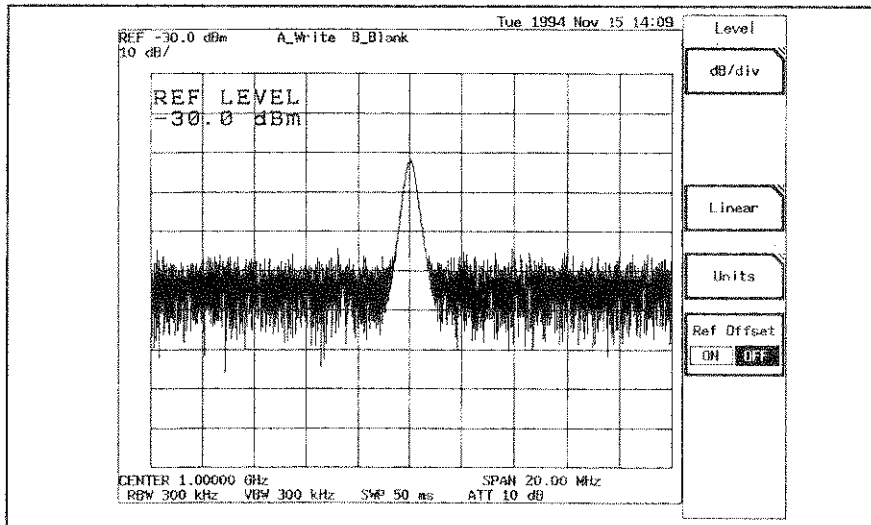
Figure 7-7 VBW = 300 kHz
