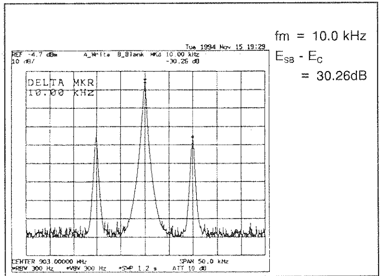
Figure 5-9 AM wave of high modulation frequency and low modulation index
