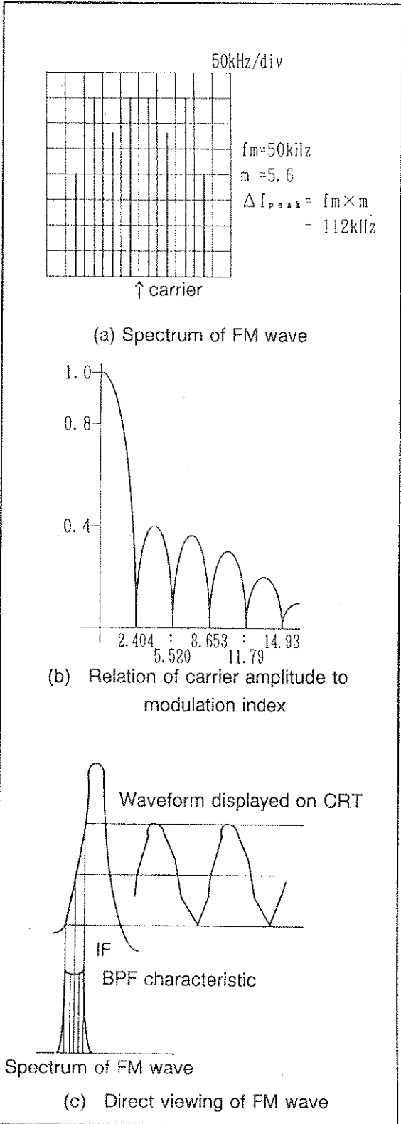
Figure 5-11 Measurement of FM wave
