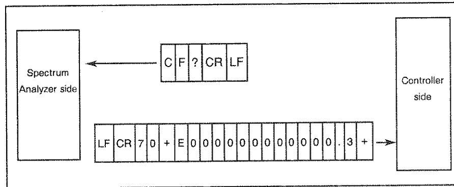
Figure 8-6 Data format
